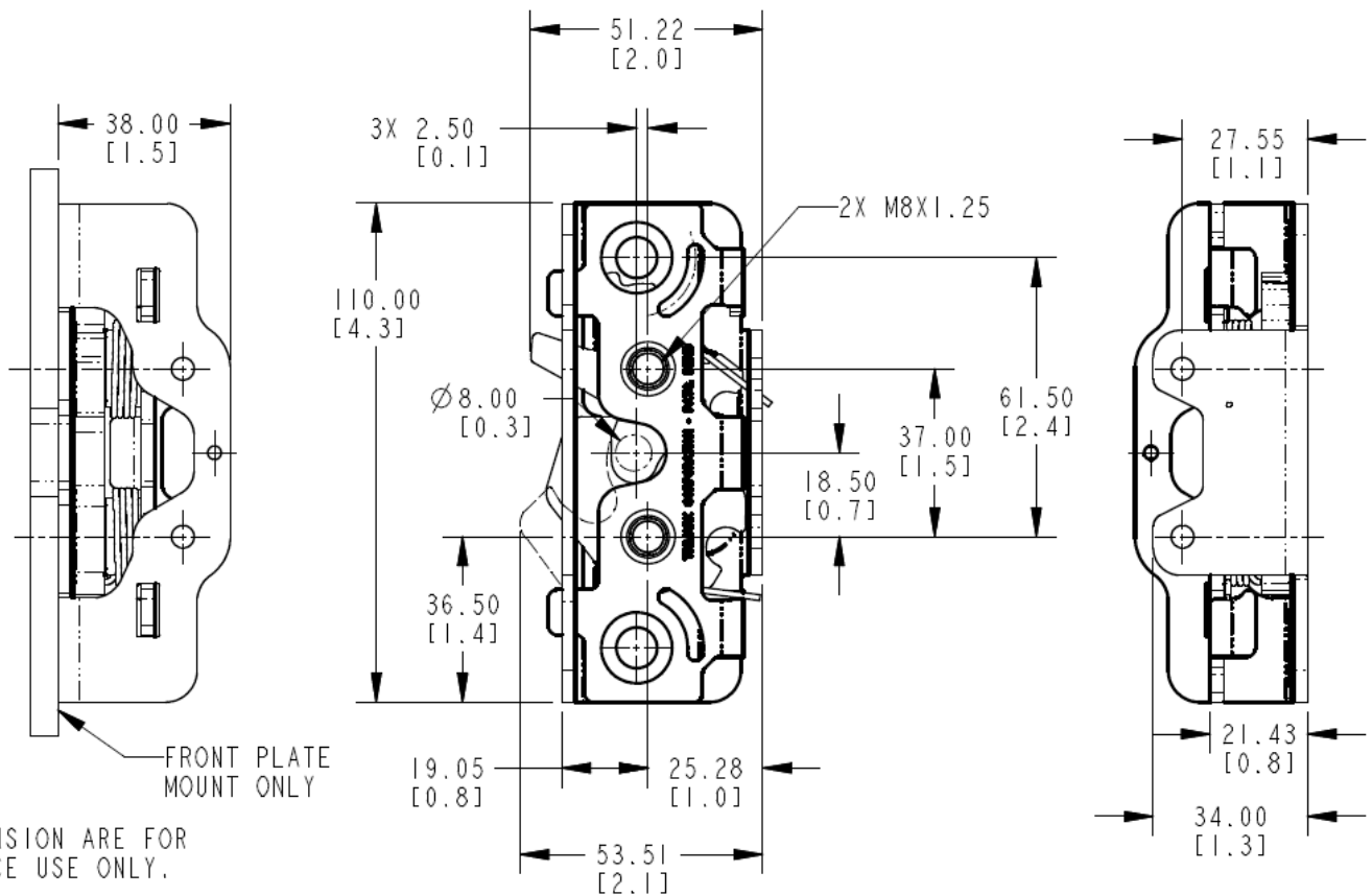
Base Latch Shown Without Actuators
